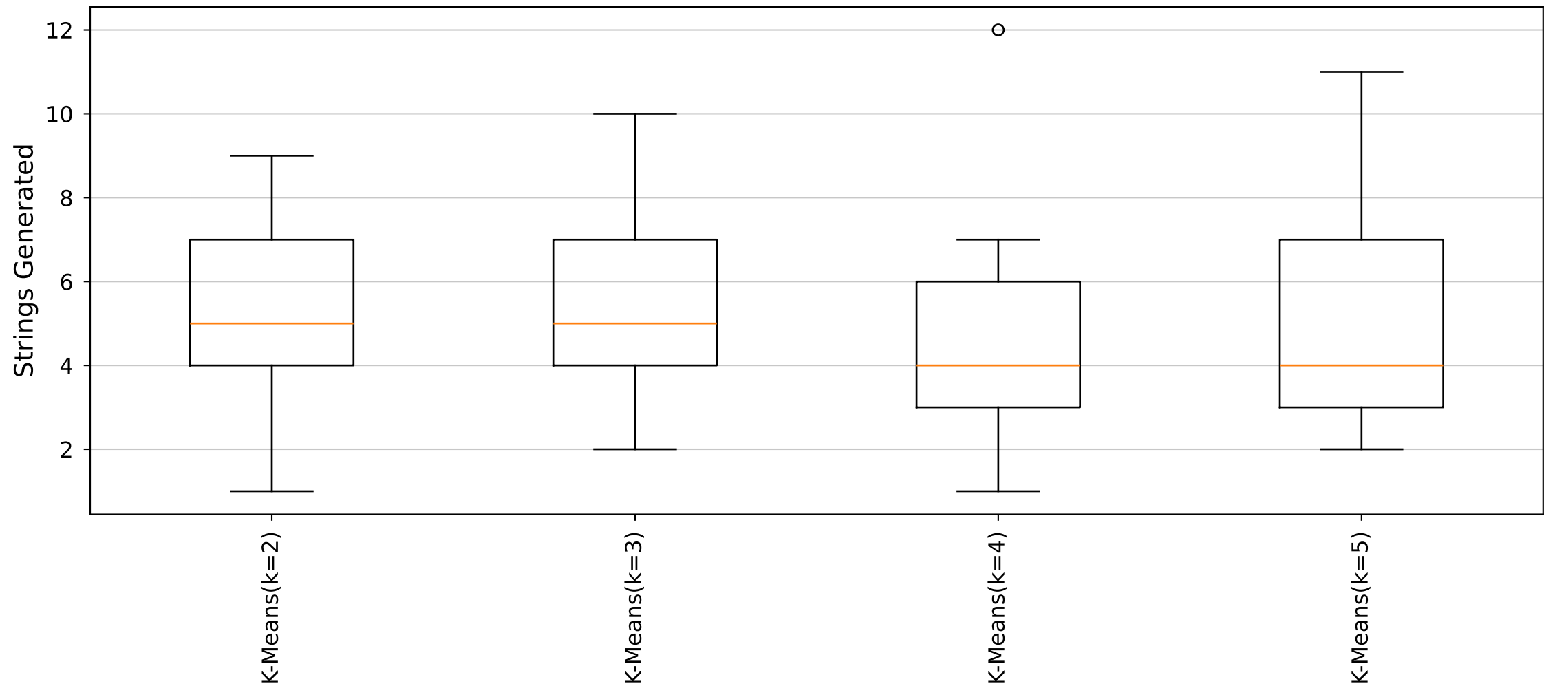
YARA Rules Strings Generated Distribution (Cluster43_Size5 dataset)
